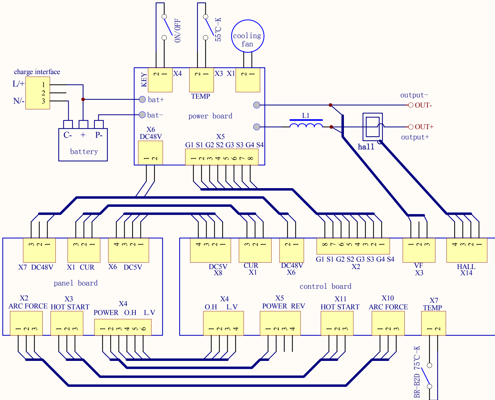
Operating principle block diagram of circuit
