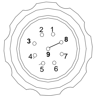
CONECTOR AEREO VISTA EXTERIOR
